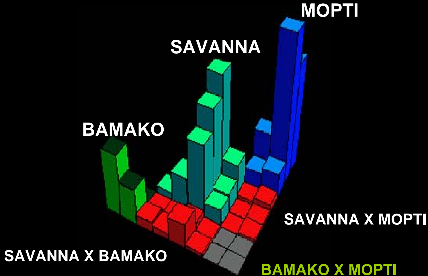
Figure 5. The distribution of inversion karyotypes observed in the village of Banambani In Mali (west Africa). The observed distribution suggests the existence of 3 sympatric subpopulations among which gene flow is restricted or absent. These subpopulations are referred to as “chromosomal forms” and have been given the names Bamako, Savanna and Mopti forms. Adapted from Touré et al. 1998
